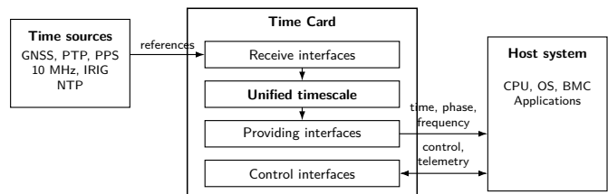
Fig. 1. Time Card context: external references enter through receive interfaces, discipline one unified timescale, and reach the host through providing and control interfaces.
